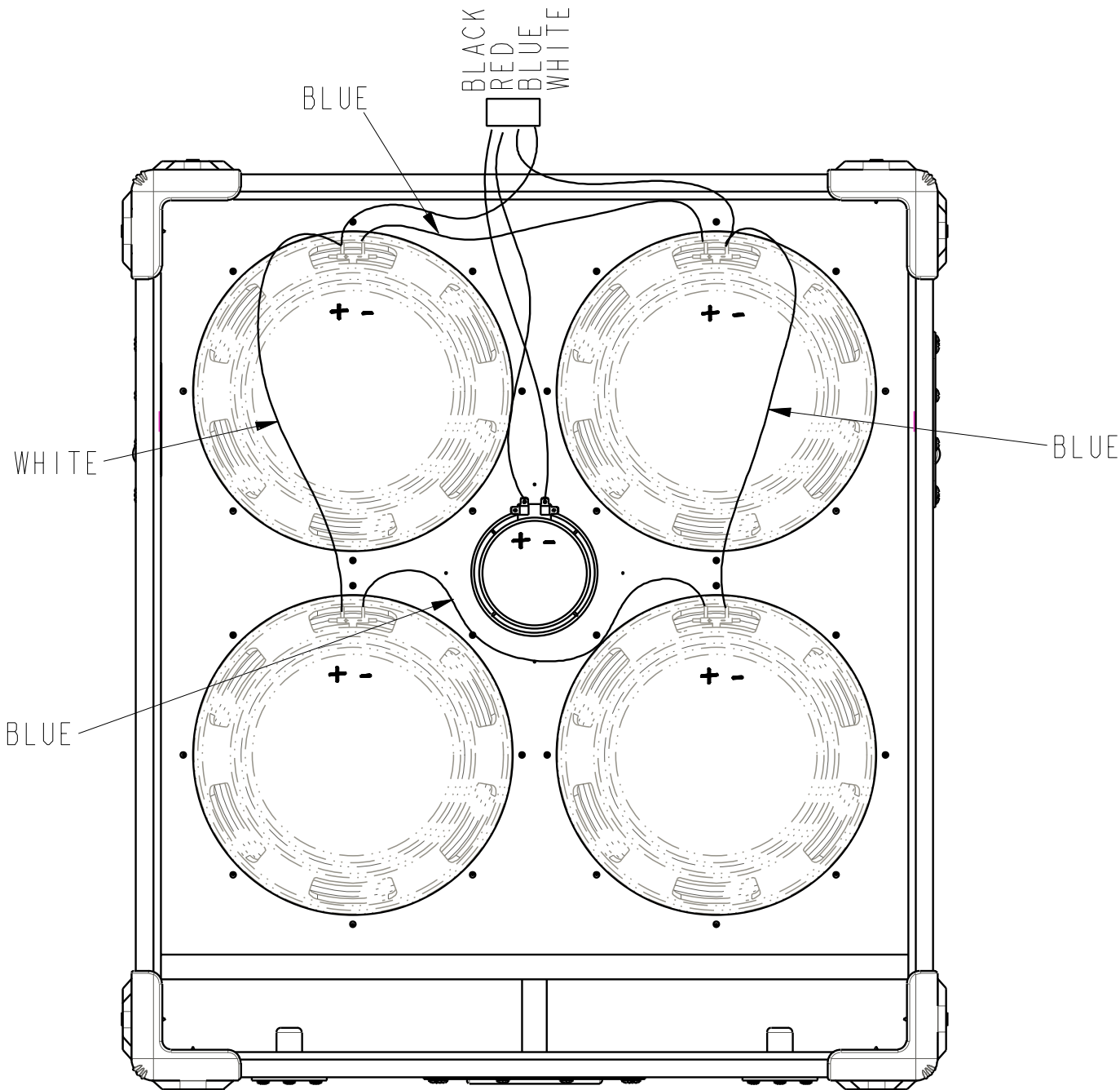
BXT41OHL4 SPEAKER HOOKUP
