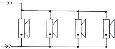
16Ω SPEAKERS (4) SST ONLY
