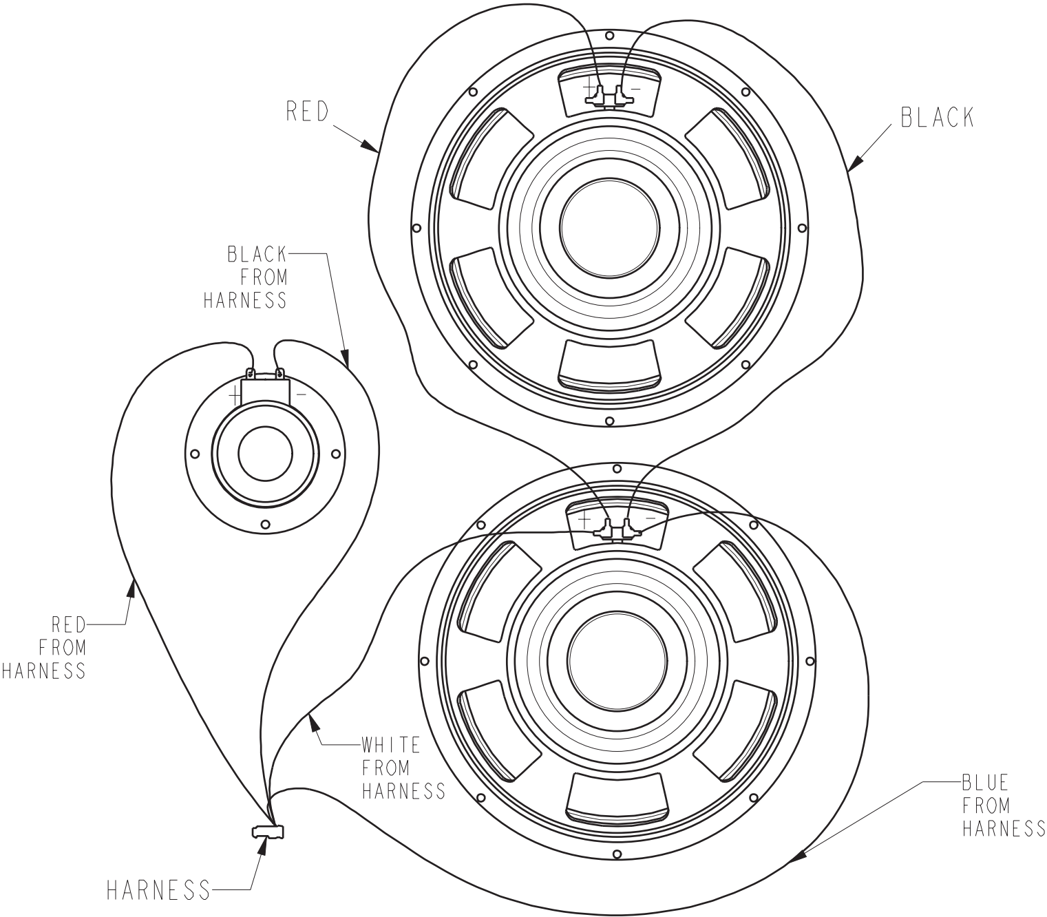
DETAIL (C) SPEAKER ORIENTATION/HOOKUP
