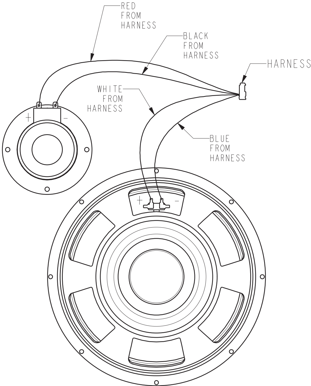
DETAIL (C) SPEAKER ORIENTATION/HOOKUP
