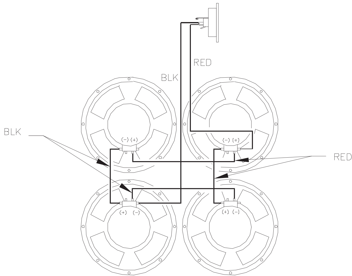
LOOKING INSIDE OF CABINET
