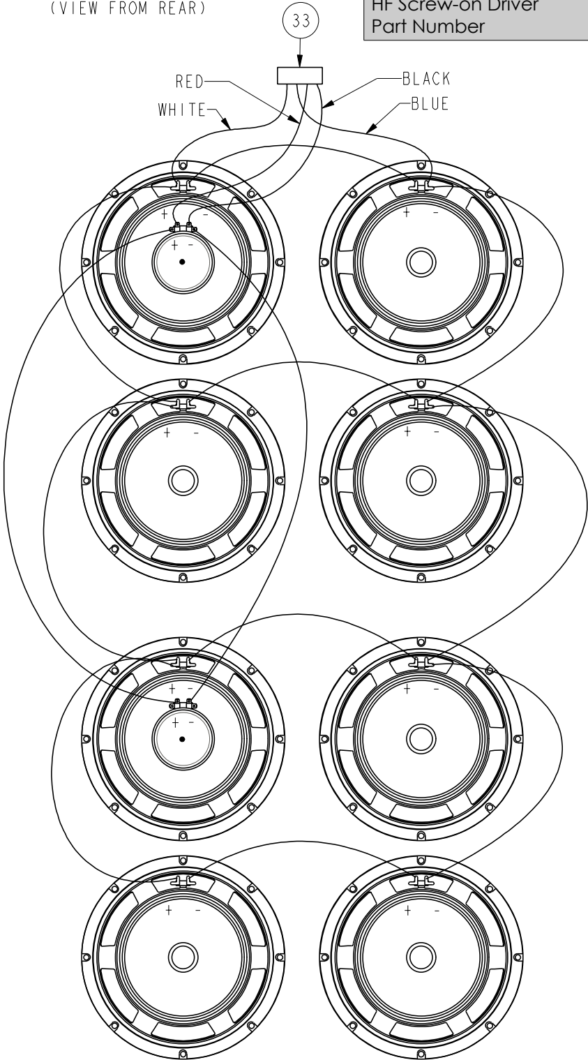
SPEAKER PLACEMENT / HOOKUP (VIEW FROM REAR)
