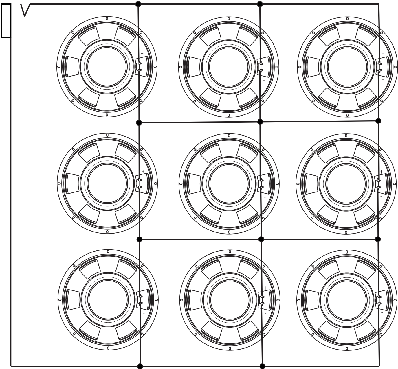
V9 ENCLOSURE
