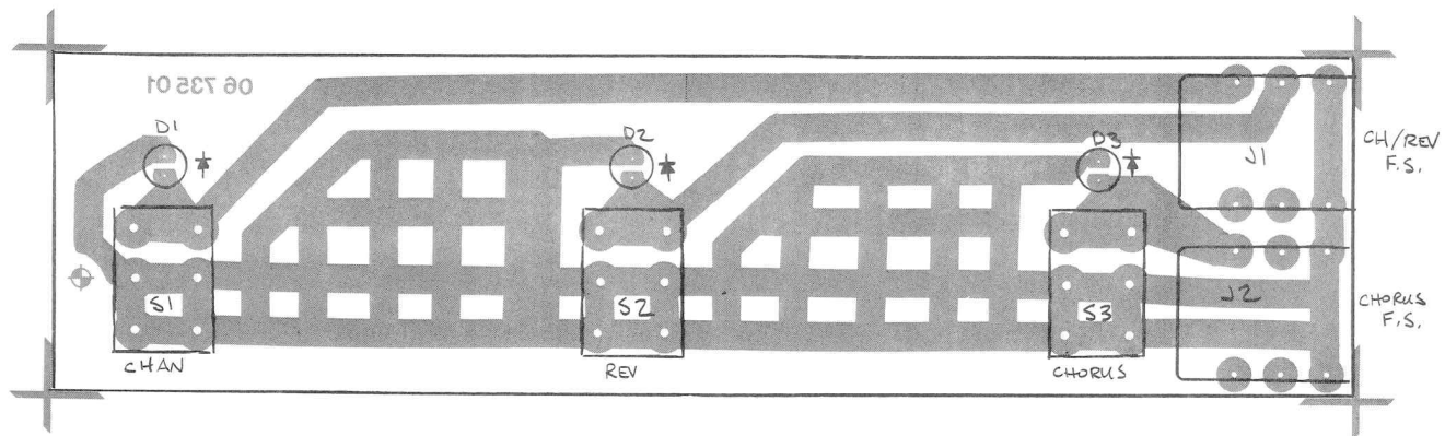
AFP-3 P.C. BOARD ASSEMBLY #07-735-01
