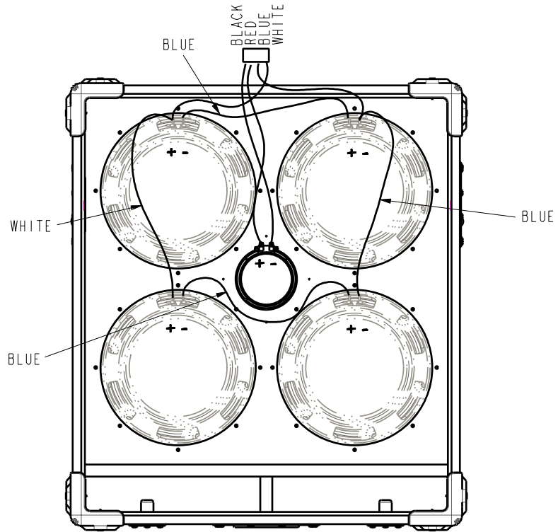
BXT41OHL4 SPEAKER HOOKUP
