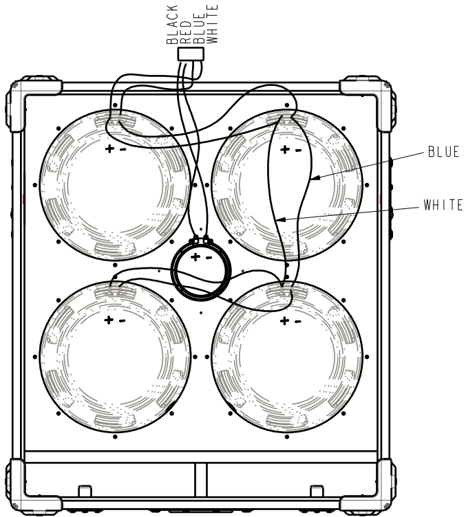
BXT41OHL8 SPEAKER HOOKUP
