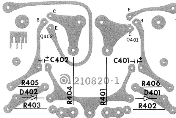
POWER SUPPLY P.C. BOARD (VIEWED FROM COPPER SIDE)
